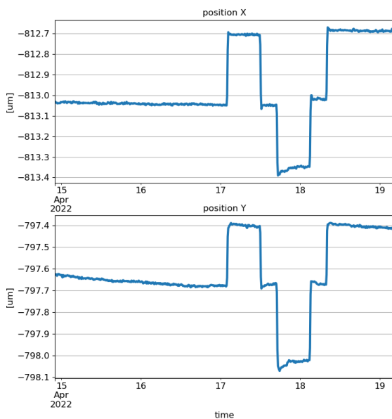
Figure 8: A four-day test in the temperature chamber.
