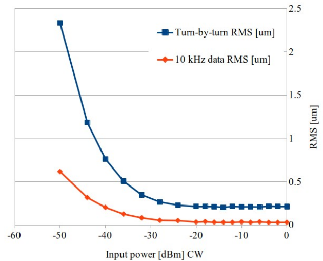
Figure 5: The turn-by-turn RMS and 10 kHz data RMS values are < 1 \mu m down to -40 dBm CW input signal.
