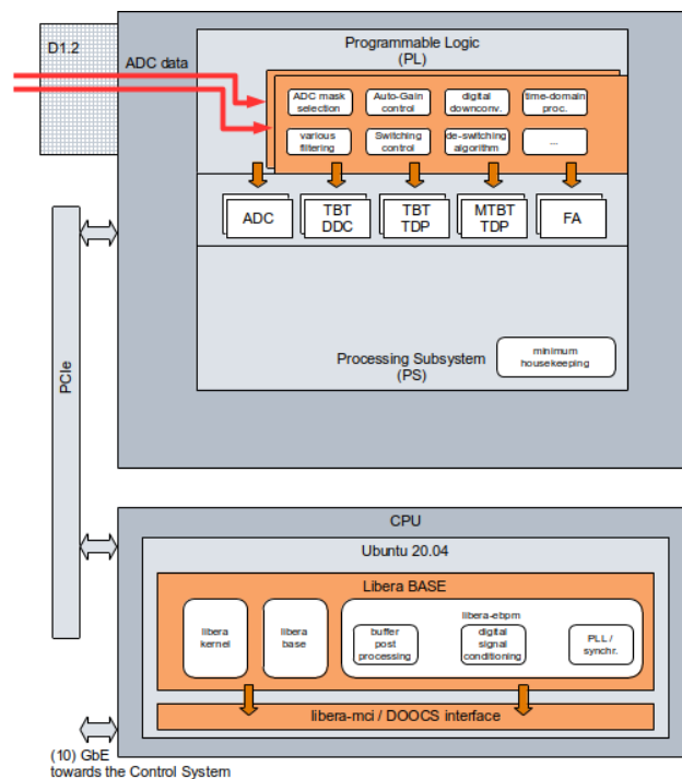
Figure 3: Signal processing, data buffers and software framework in the AMC and the CPU modules.
