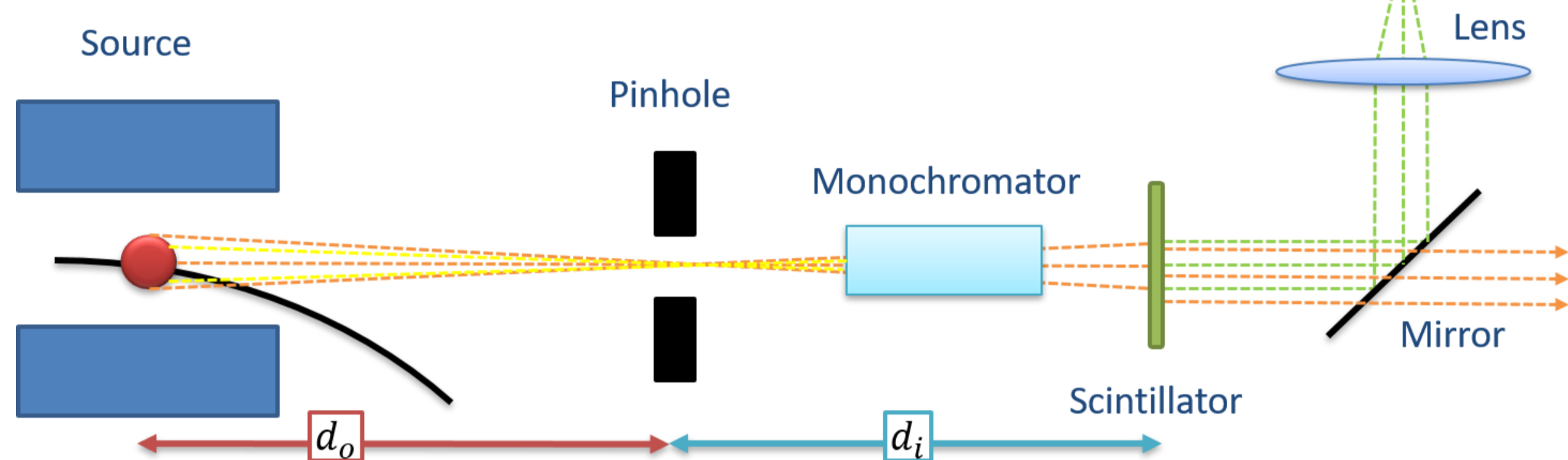
Figure 1: Schematic of the monochromatic X-ray pinhole camera system.
